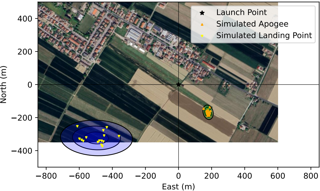
1 \sigma , 2 \sigma and 3 \sigma Dispersion Ellipses: Apogee and Landing Points
